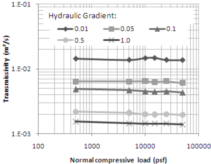
Figure 6: Effect of normal load on the transmissivity of “Draintube” géocomposite
