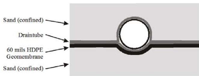
Figure 5 : Test configuration
