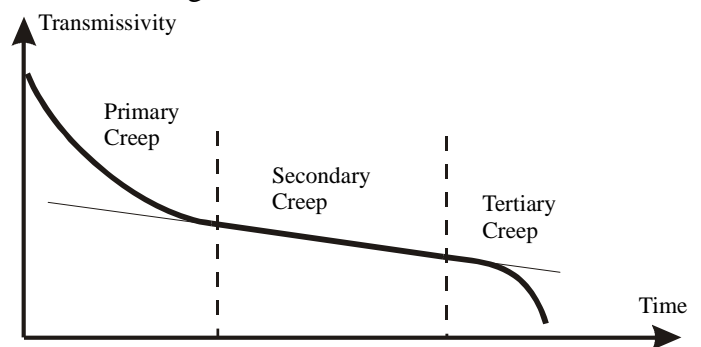
Figure 4: Creep behavior of planar drainage geosynthetics
