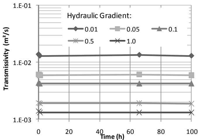
Figure 7: Effect of time on the transmissivity of “Draintube” géocomposite
