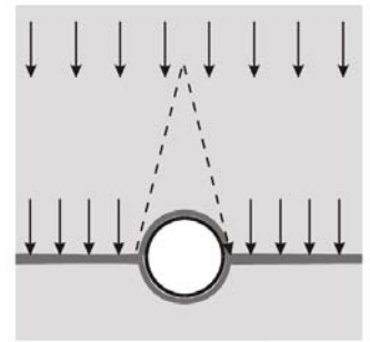
Figure 3: soil arching effect
