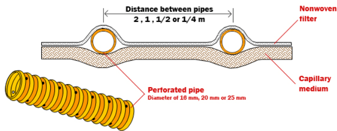
Figure 1 : Drain Tubes geocomposite Description
